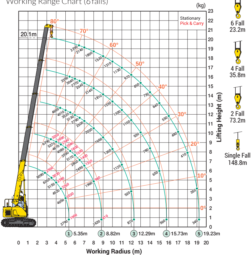
Working Range Chart (6 falls)
